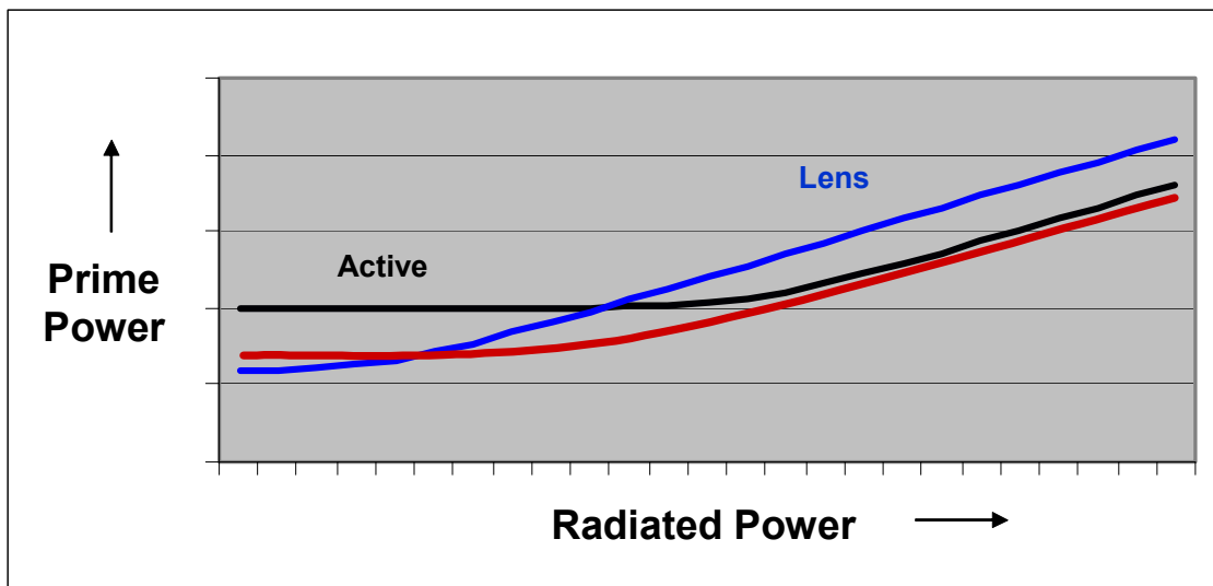
Fig. 7. Notional radiated power efficiency for passive lens (Lens), a constrained-feed active ESA (Active), and the active lens (Active Lens). At low radiated power, the Lens is most efficient due to lowest number of receivers. At low power, the Active Lens is less efficient than the passive lens, but more efficient than the Active ESA due to the greater efficiency of space feed versus constrained feed. At high radiated power, overhead power is no longer dominant and the passive lens suffers due to the losses on transmit and receive. The Active Lens and Active ESA are approximately the same.
